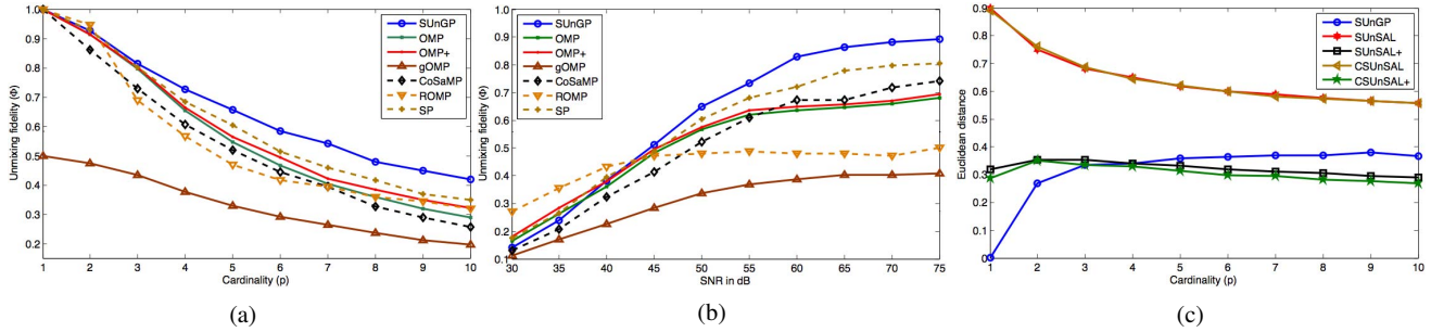
Fig. 2: Comparison of the results on synthetic data: a) Unmixing fidelity computed by different algorithms, as a function of the cardinality of the mixed pixels. The image contains the Gaussian white noise with \text{SNR} = 50\text{dB} for each pixel. b) Unmixing fidelity as a function of the SNR of the pixels. The cardinality of each pixel is 5. c) Euclidean distance between \alpha_0 and \hat{\alpha} , as a function of the cardinality of the mixed pixels. The comparison is between SUnGP and the convex relaxation based algorithms.
