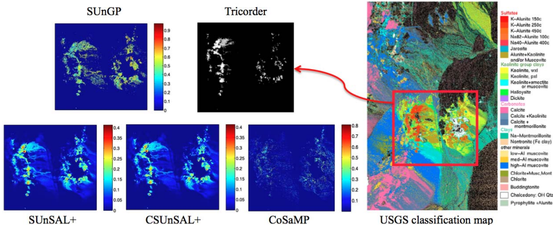
Fig. 3: Comparison of the results on the real-world data : The USGS classification map shows the labels of different materials in an image taken over Cuprite mines, NV. The labels are assigned with the Tricorder software. The 350 \times 350 area inside the rectangle is analyzed in this work. The Tricorder map shows the classification map of Alunite (a mineral) in the region. Each of the other four maps show the fractional abundances of Alunite in the region, computed by the algorithms mentioned.
