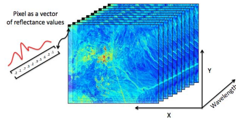
Fig. 1: Illustration of a hyperspectral image cube: The XY-plane shows the spatial dimensions and the wavelength axis shows the spectral dimension. Pixels are recorded as vectors of reflectance values at different wavelengths. The cube shows reflectance patterns at ten wavelength bands. The data is collected by NASA's AVIRIS [12] over the Cuprite mines, NV.
